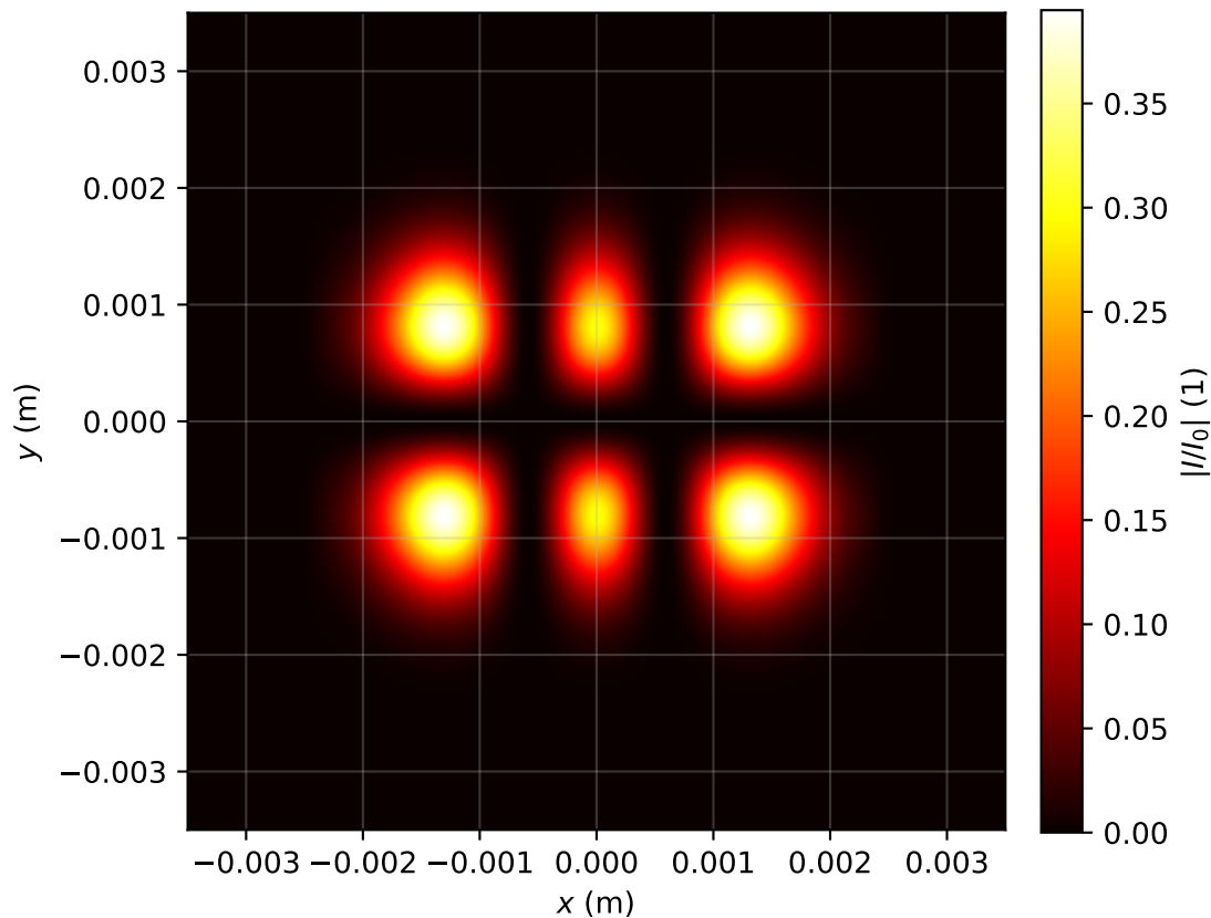
Intensity profile I(x, y, z = 2.627)/I_0 , P_{in}=0.5P_{cr} , artificial time
